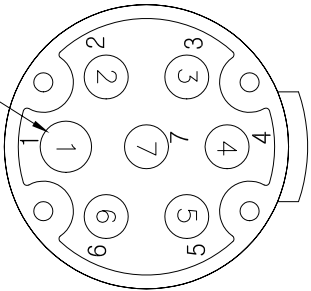
VIEW A-A SOLDER VIEW
